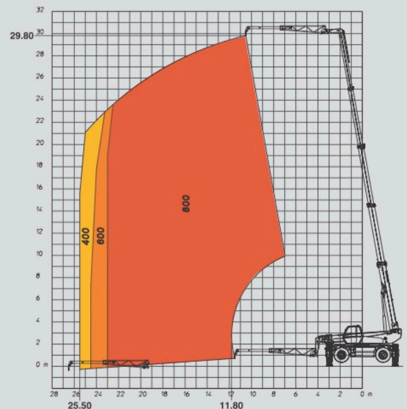
ROTATION ON STABILIZERS FULLY EXTENDED WITH TELESCOPED PT 800 JIB
